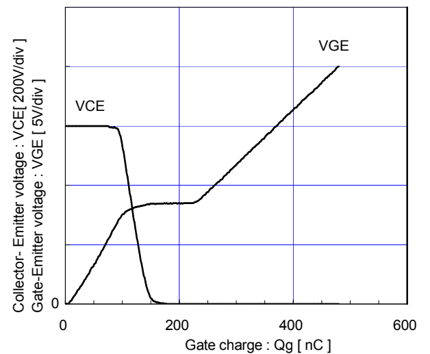
Dynamic Gate charge (typ.) Vcc=600V, Ic=100A, Tj=25°C
