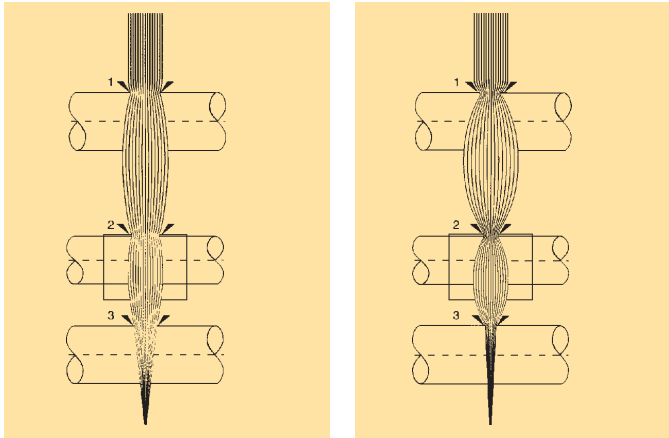
Fig. K: Correct opening width (left) and too narrow opening width (right) of condenser
