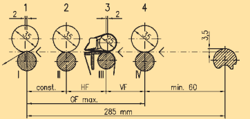
Fig. F: Draft field settings PK 5000
